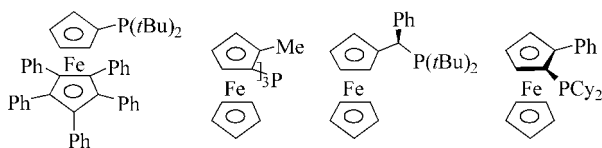
Figure 1. Ferrocenylphosphanes.
