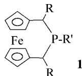
Figure 2. 2-Phospha[3]ferrocenophane derivatives 1 .
