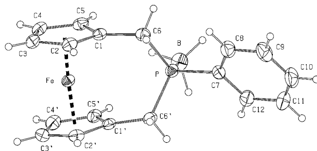
Figure 4. ORTEP view of the 2-phenyl-2-phospha[3]ferrocenophane borane complex 3c . Displacement ellipsoids are shown at the 30% probability level.
