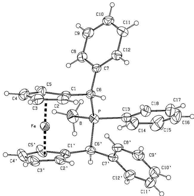
Figure 3. ORTEP drawing of dl - 3a . Displacement ellipsoids are shown at the 30% probability level.
