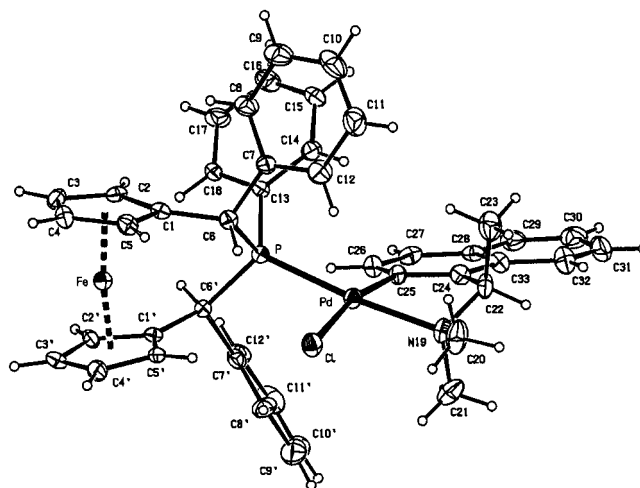
Figure 5. ORTEP view of the cyclopalladate complex 8a . Displacement ellipsoids are shown at the 30% probability level.
